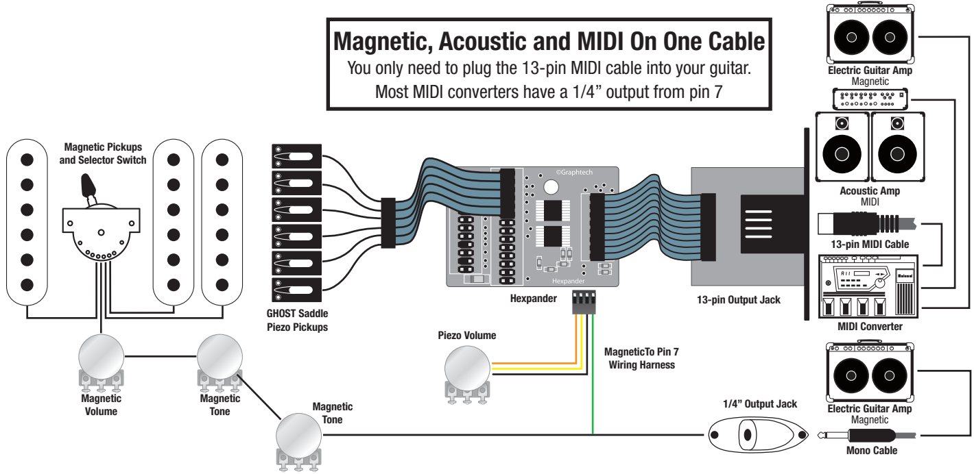
PE-0182-G0 Pin 7 Wiring Harness
