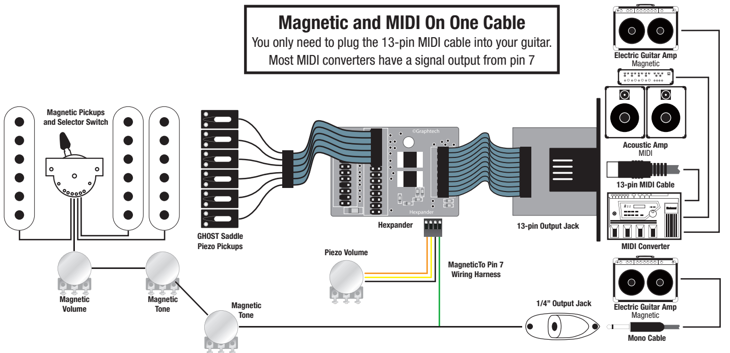
PE-0182-G0 Magnetic To Pin 7 Wiring Harness
