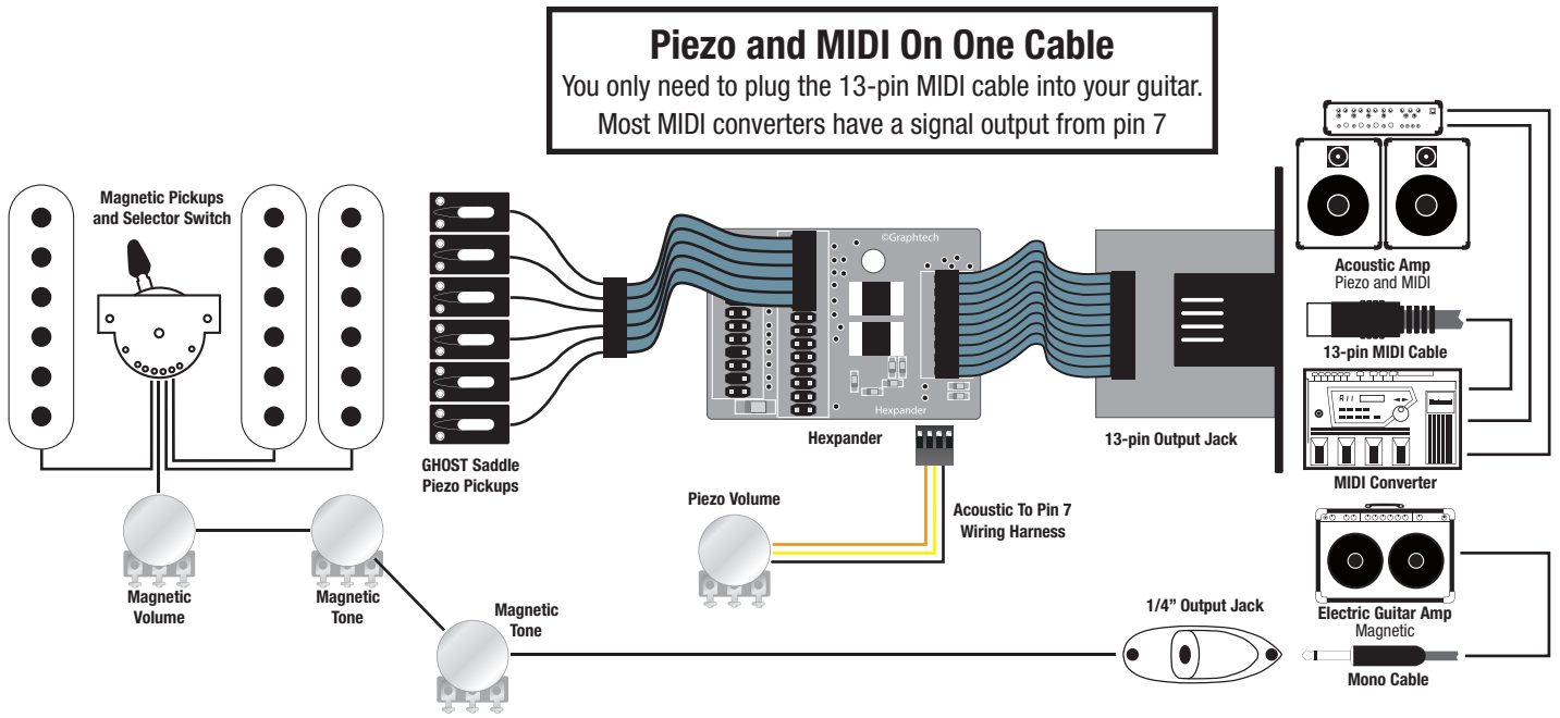
PE-0182-00 Acoustic To Pin 7 Wiring Harness
